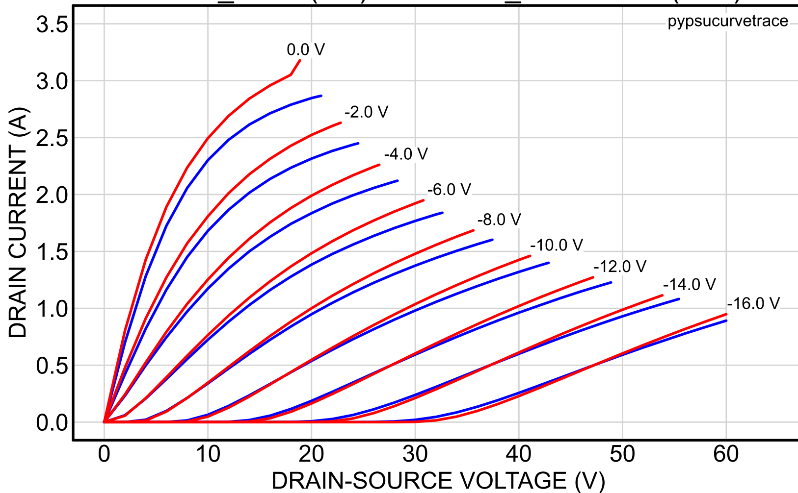
2SK82_11NA (red) vs. 2SK82_40reserved (blue)
