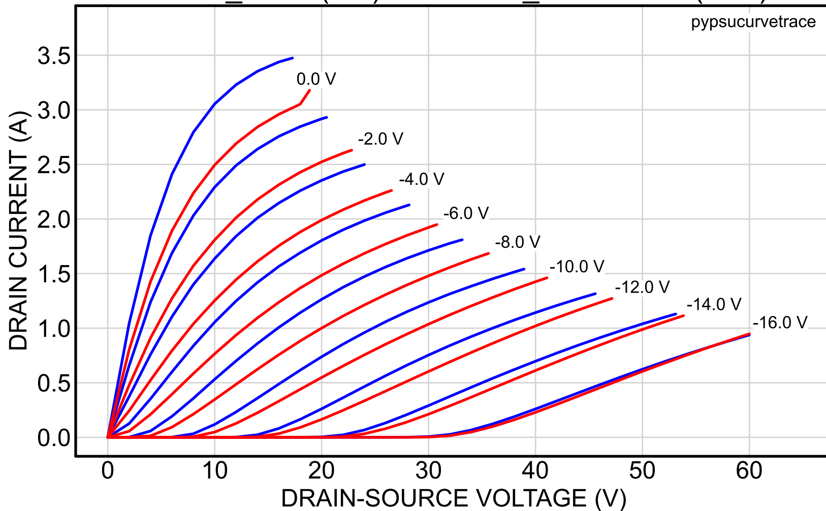
2SK82_11NA (red) vs. 2SK82_52reserved (blue)
