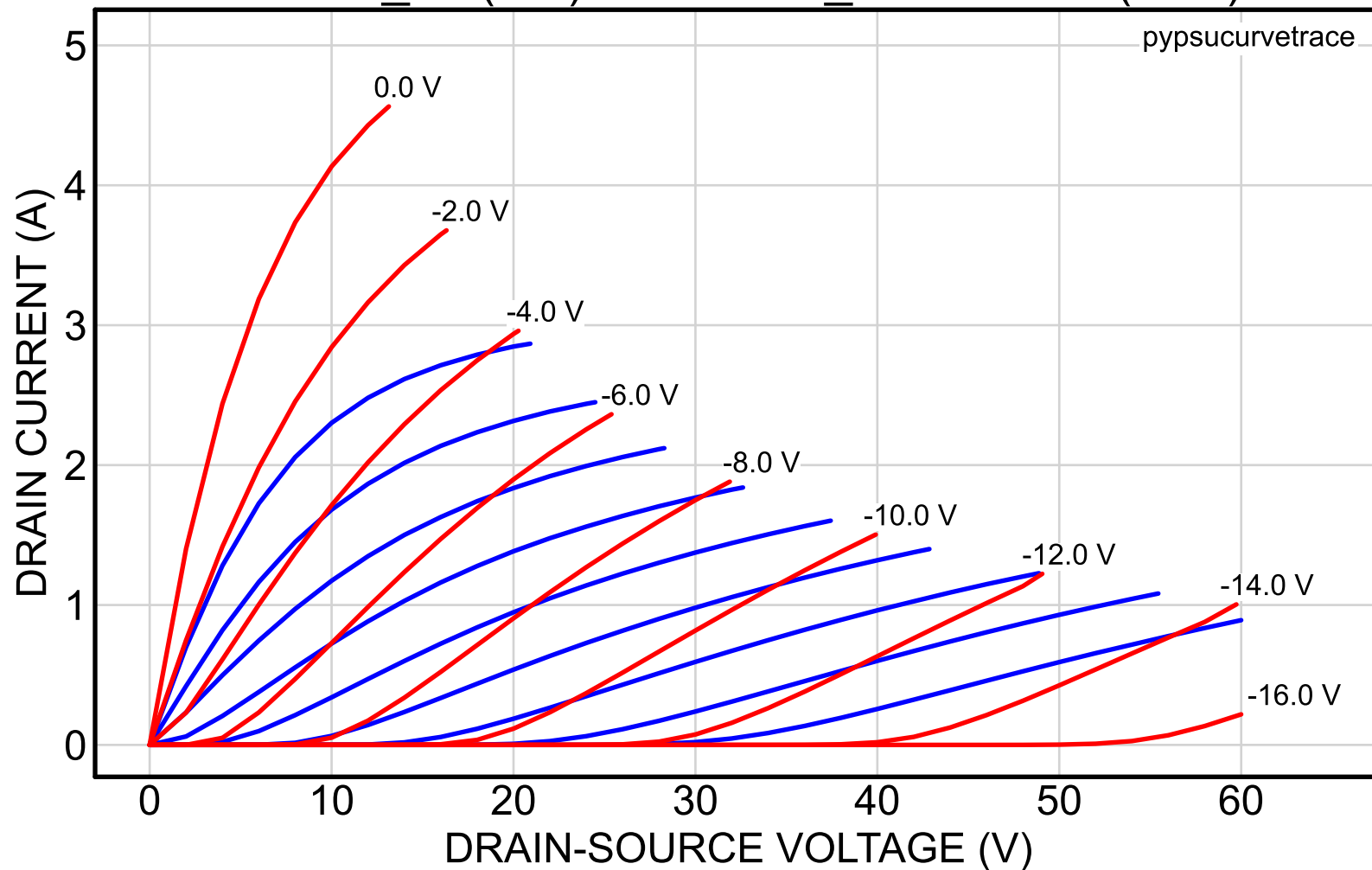
2SK82_12 (red) vs. 2SK82_40reserved (blue)
