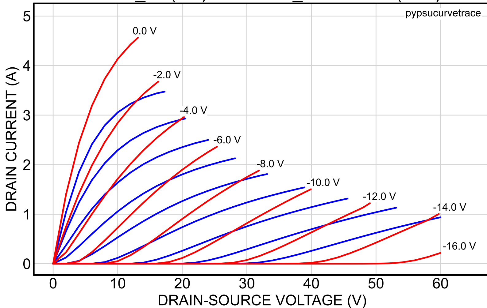
2SK82_12 (red) vs. 2SK82_52reserved (blue)
