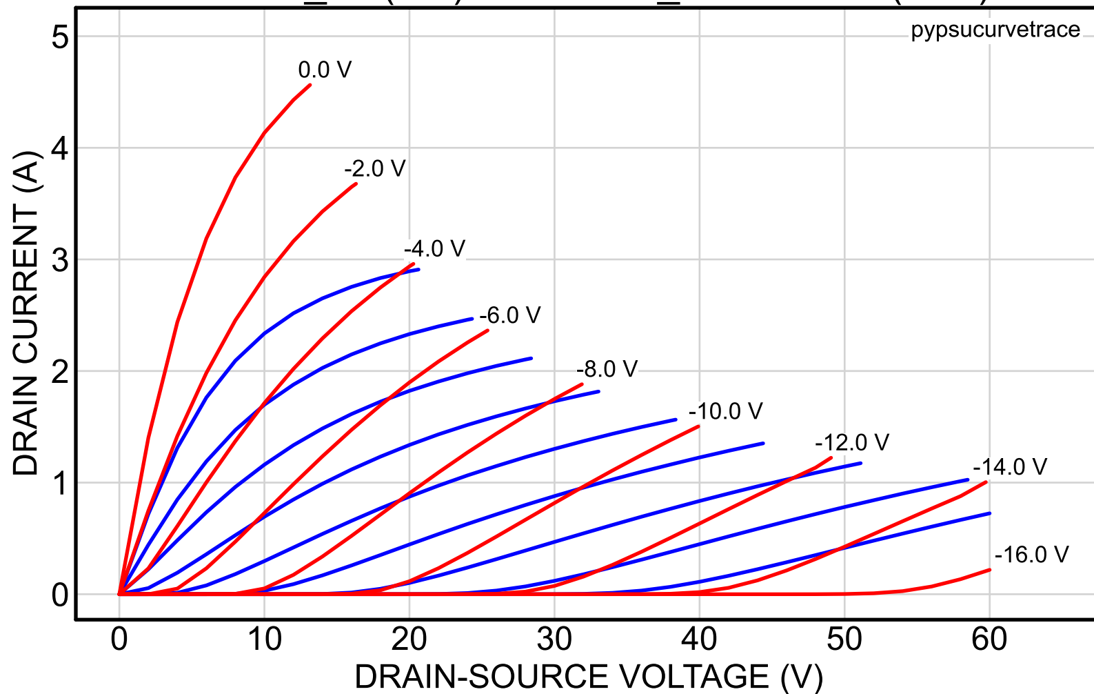
2SK82_12 (red) vs. 2SK82_56reserved (blue)
