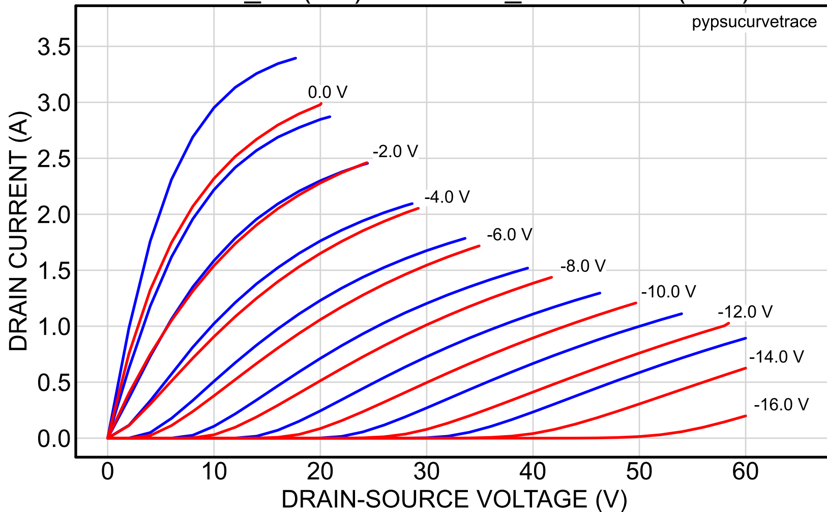
2SK82_13 (red) vs. 2SK82_39reserved (blue)
