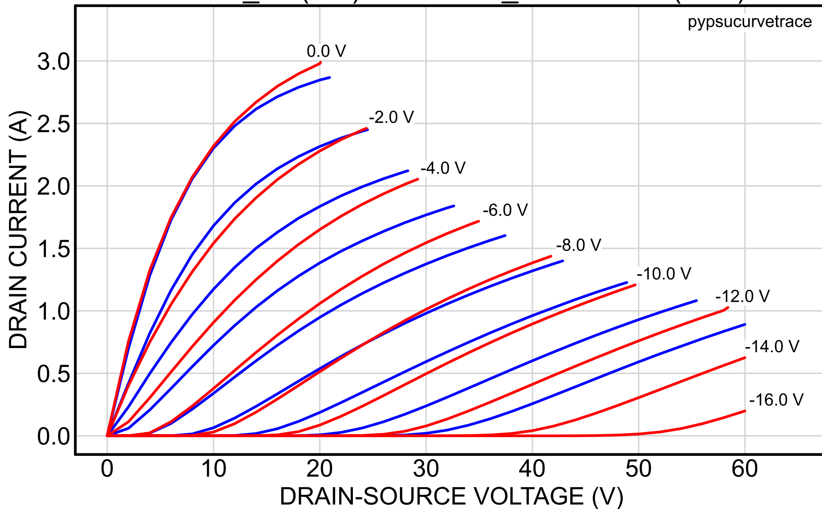
2SK82_13 (red) vs. 2SK82_40reserved (blue)
