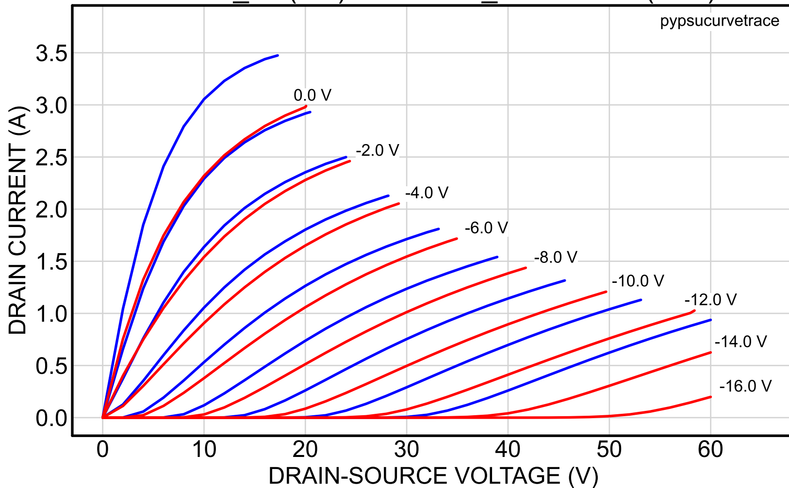
2SK82_13 (red) vs. 2SK82_52reserved (blue)
