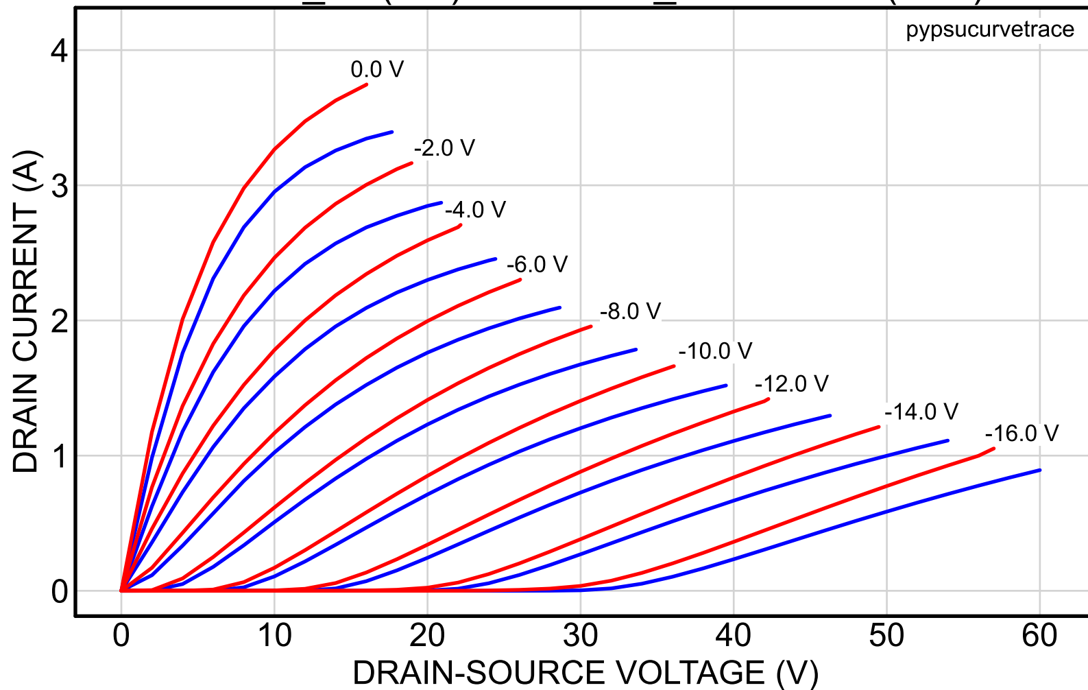
2SK82_14 (red) vs. 2SK82_39reserved (blue)
