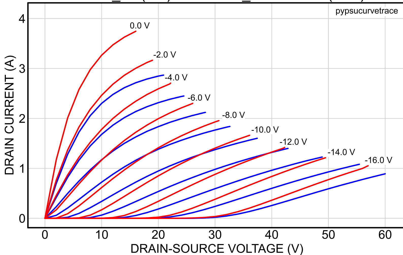
2SK82_14 (red) vs. 2SK82_40reserved (blue)
