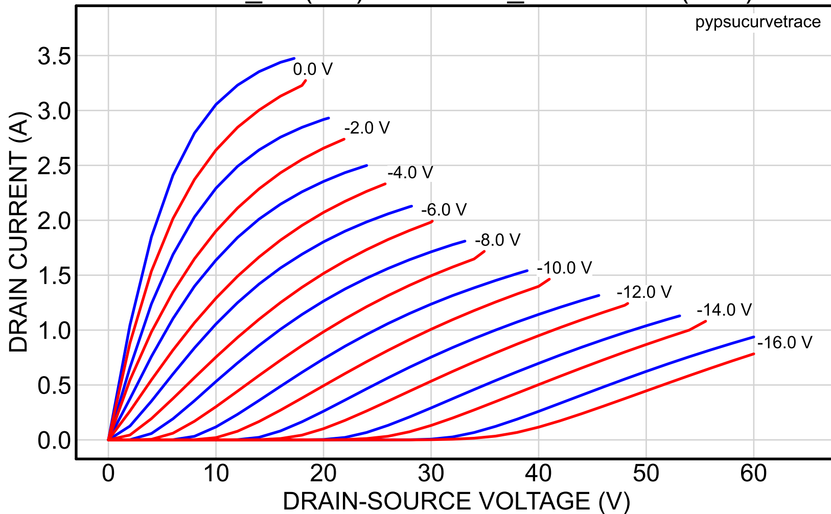
2SK82_15 (red) vs. 2SK82_52reserved (blue)
