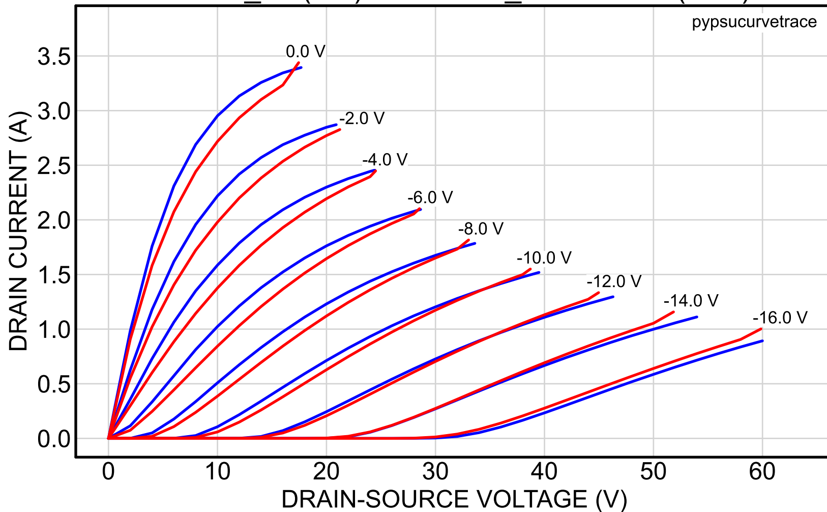
2SK82_16 (red) vs. 2SK82_39reserved (blue)
