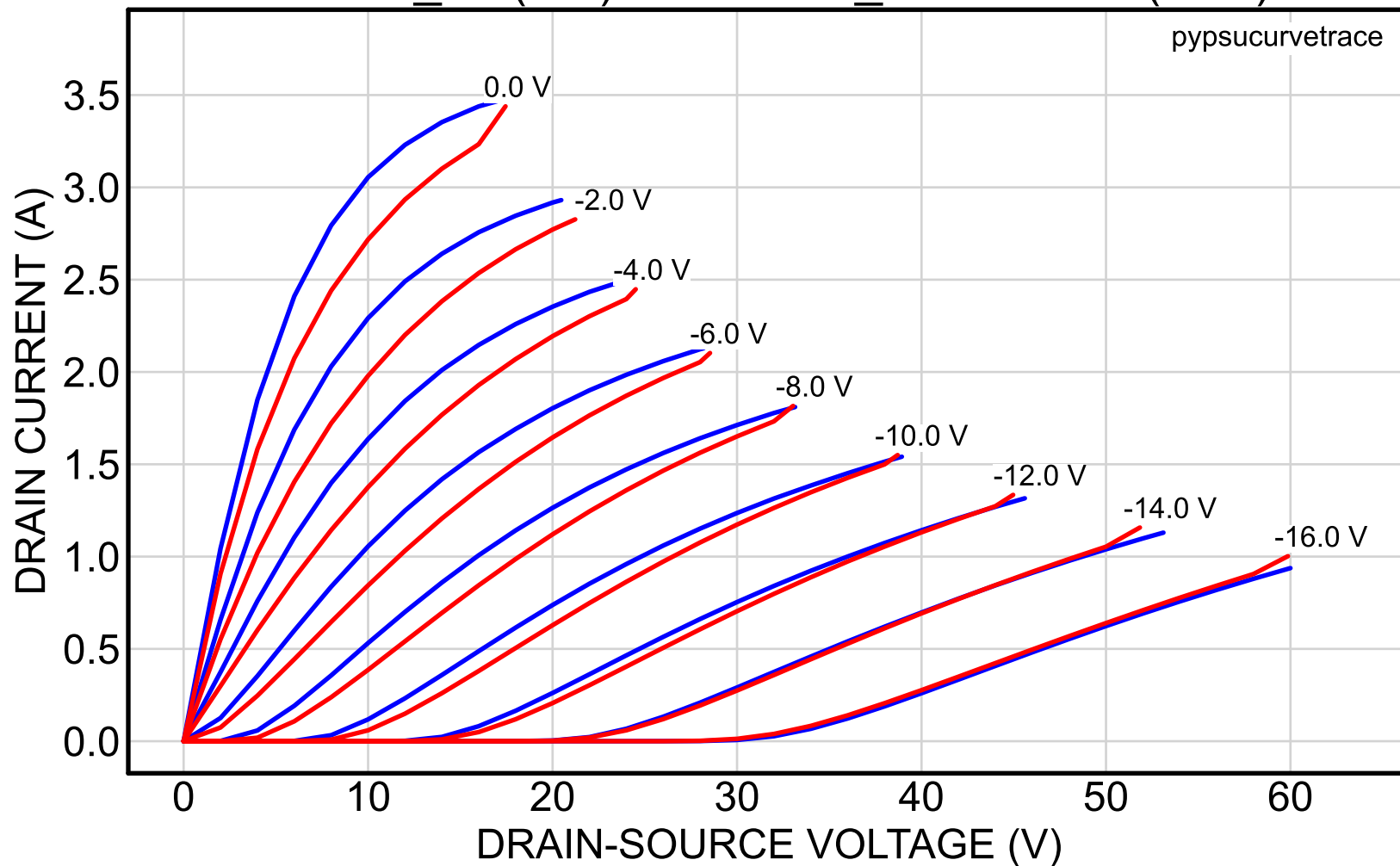
2SK82_16 (red) vs. 2SK82_52reserved (blue)
