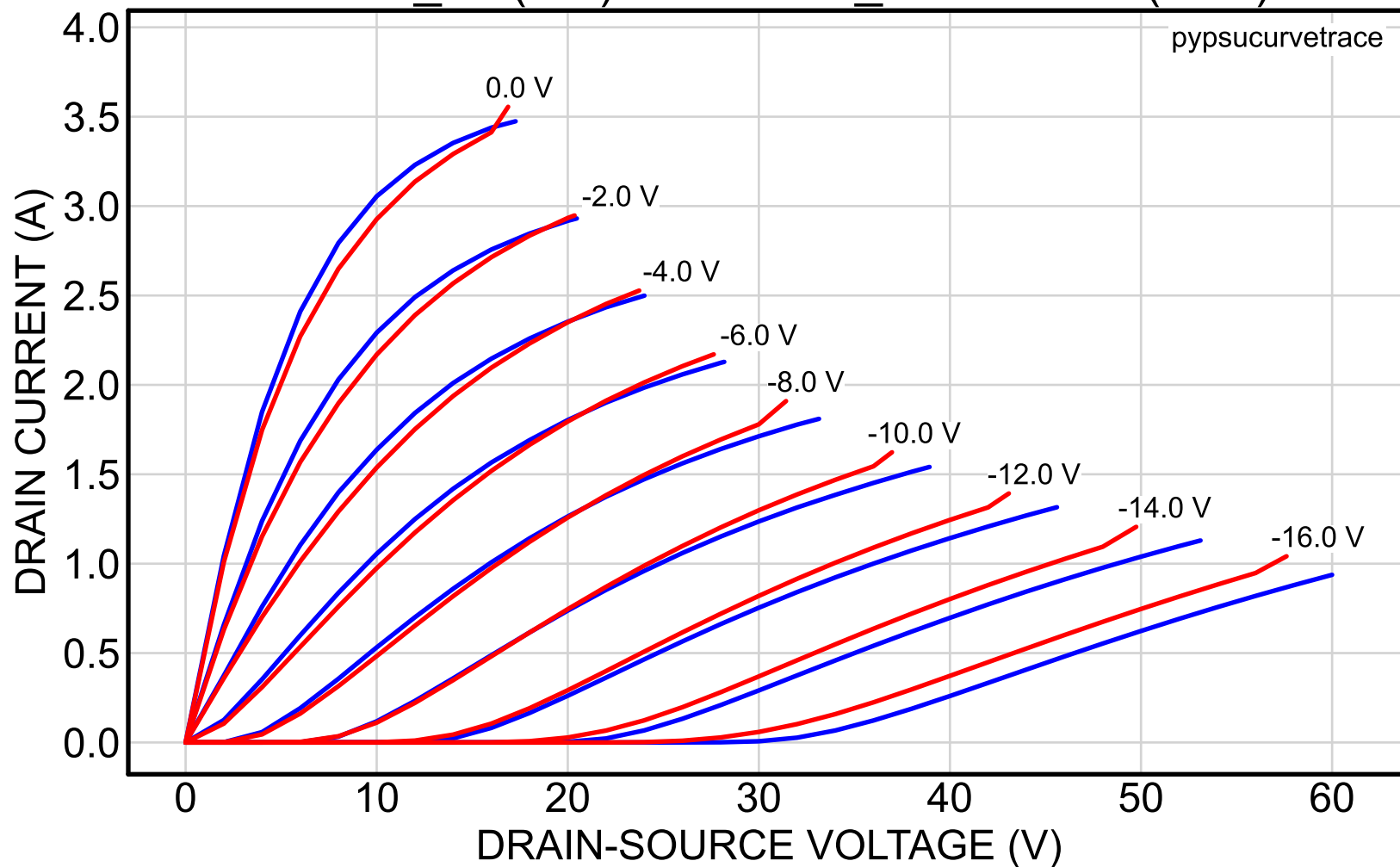
2SK82_17 (red) vs. 2SK82_52reserved (blue)
