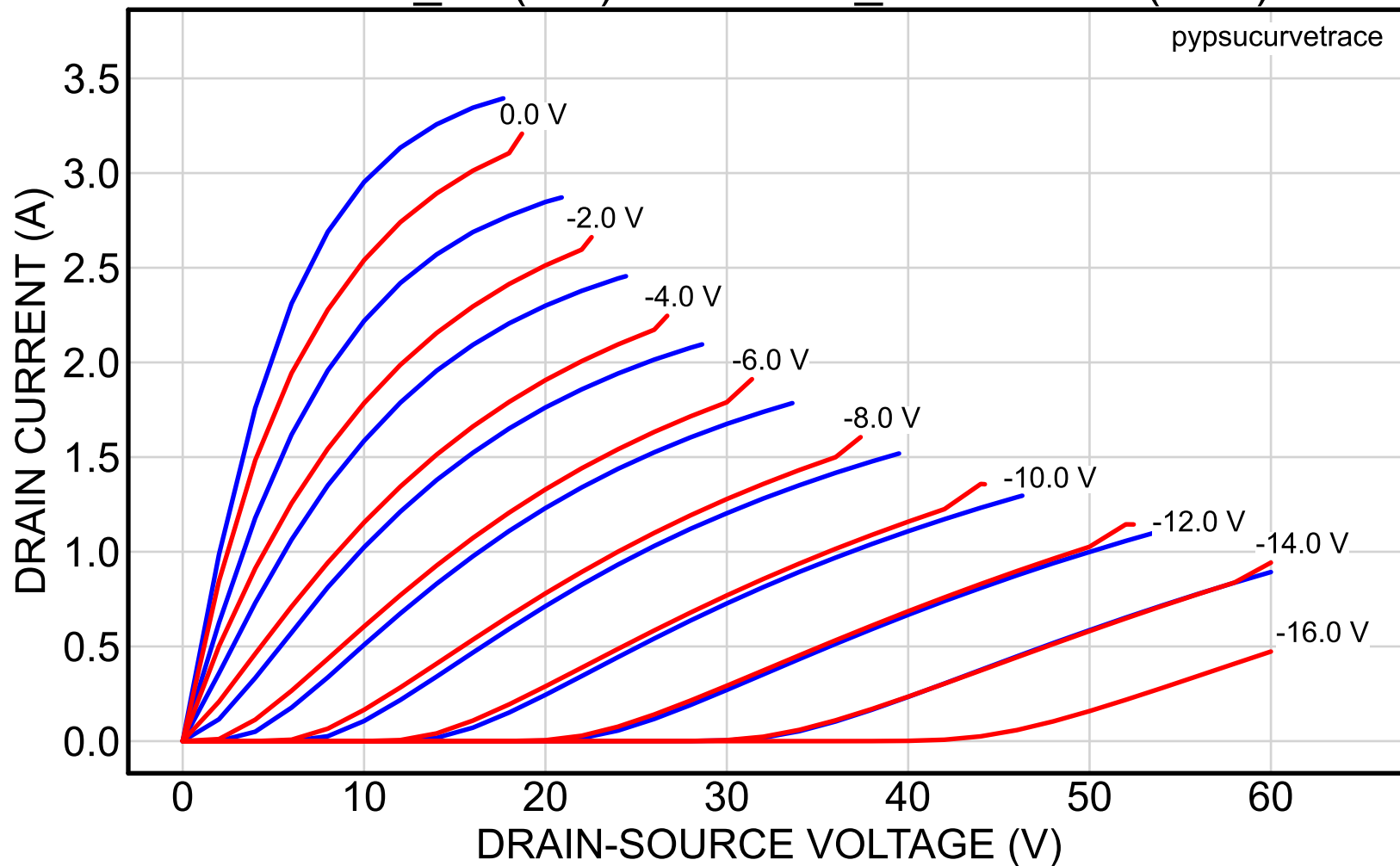
2SK82_18 (red) vs. 2SK82_39reserved (blue)
