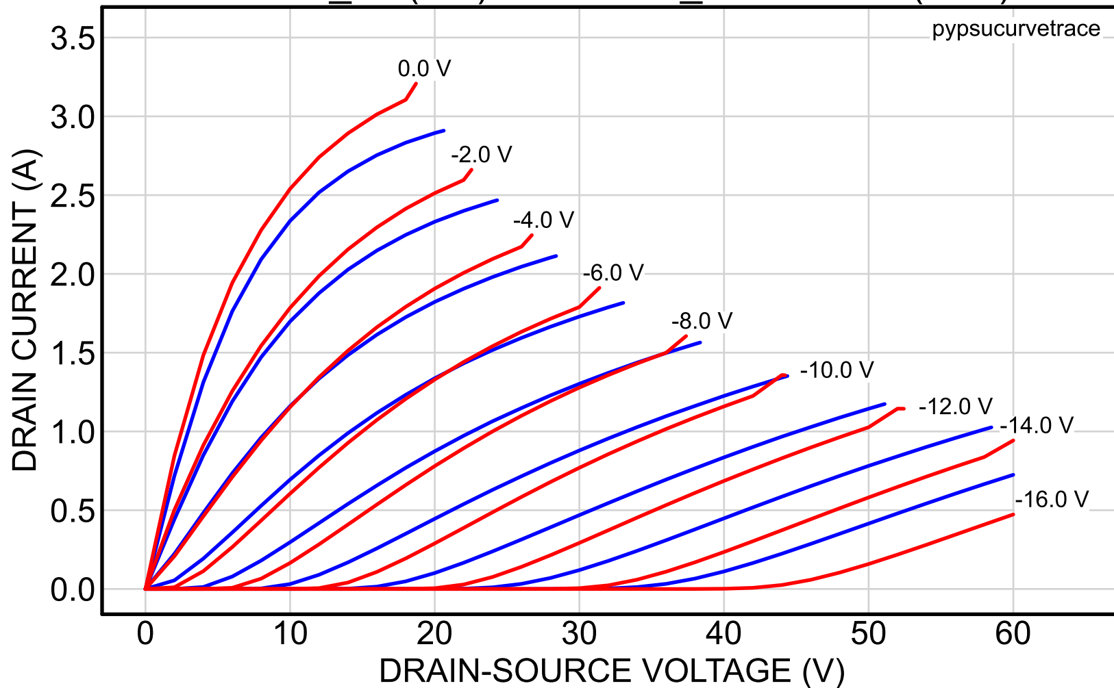
2SK82_18 (red) vs. 2SK82_56reserved (blue)
