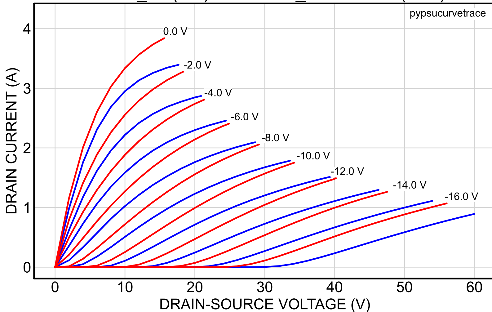
2SK82_19 (red) vs. 2SK82_39reserved (blue)
