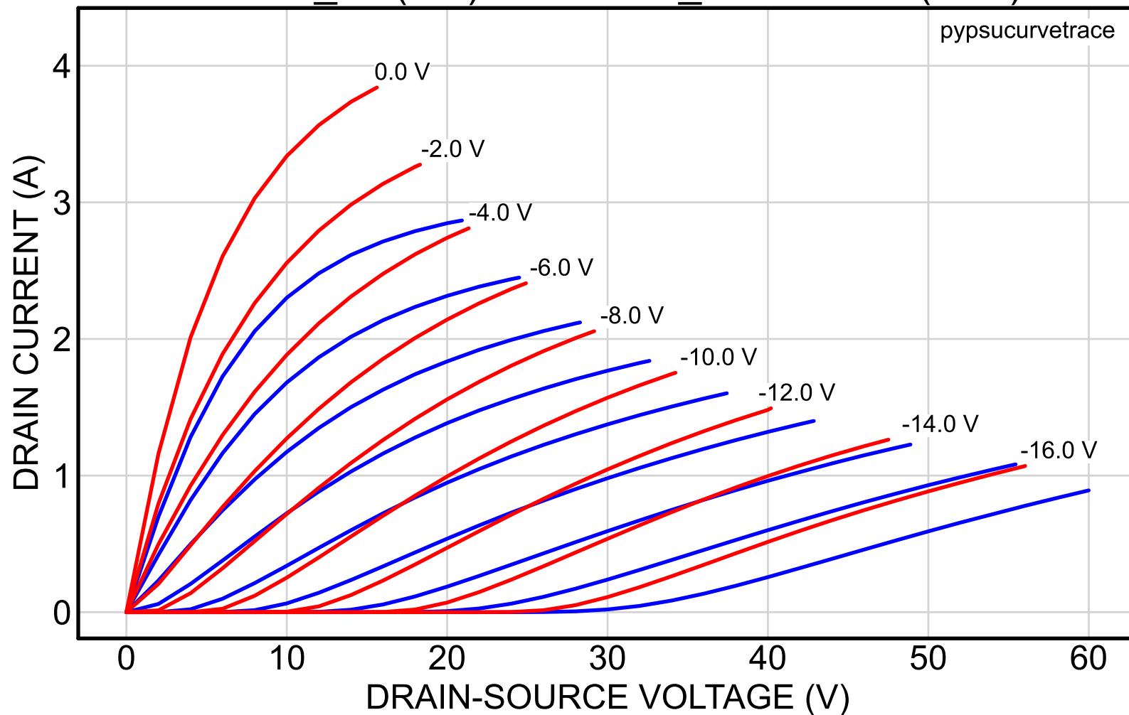
2SK82_19 (red) vs. 2SK82_40reserved (blue)
