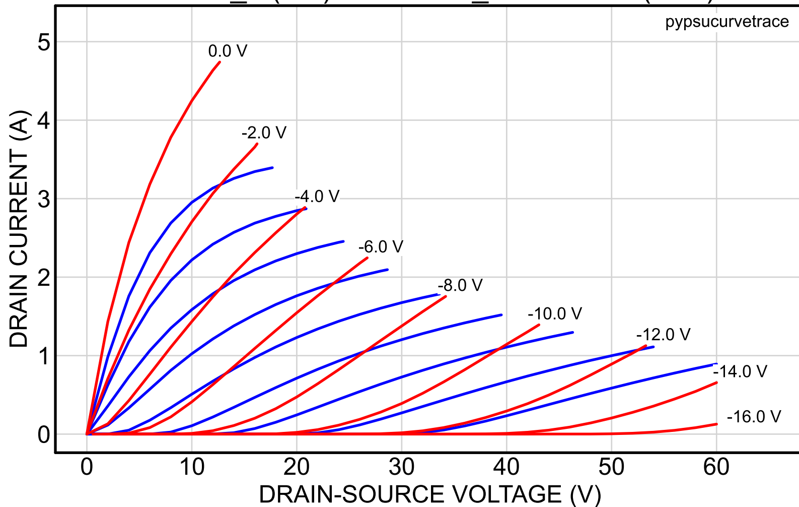
2SK82_1 (red) vs. 2SK82_39reserved (blue)
