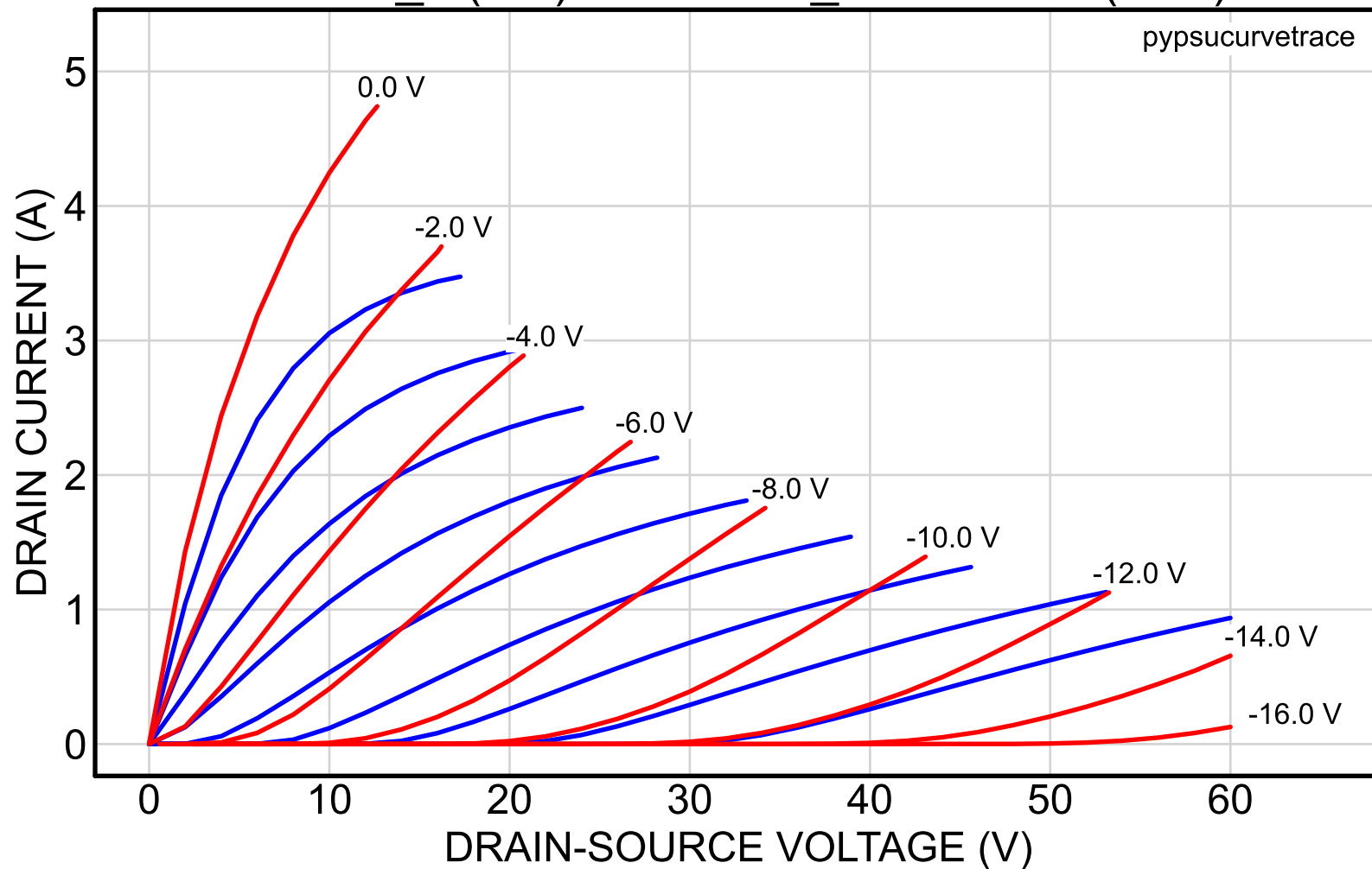
2SK82_1 (red) vs. 2SK82_52reserved (blue)
