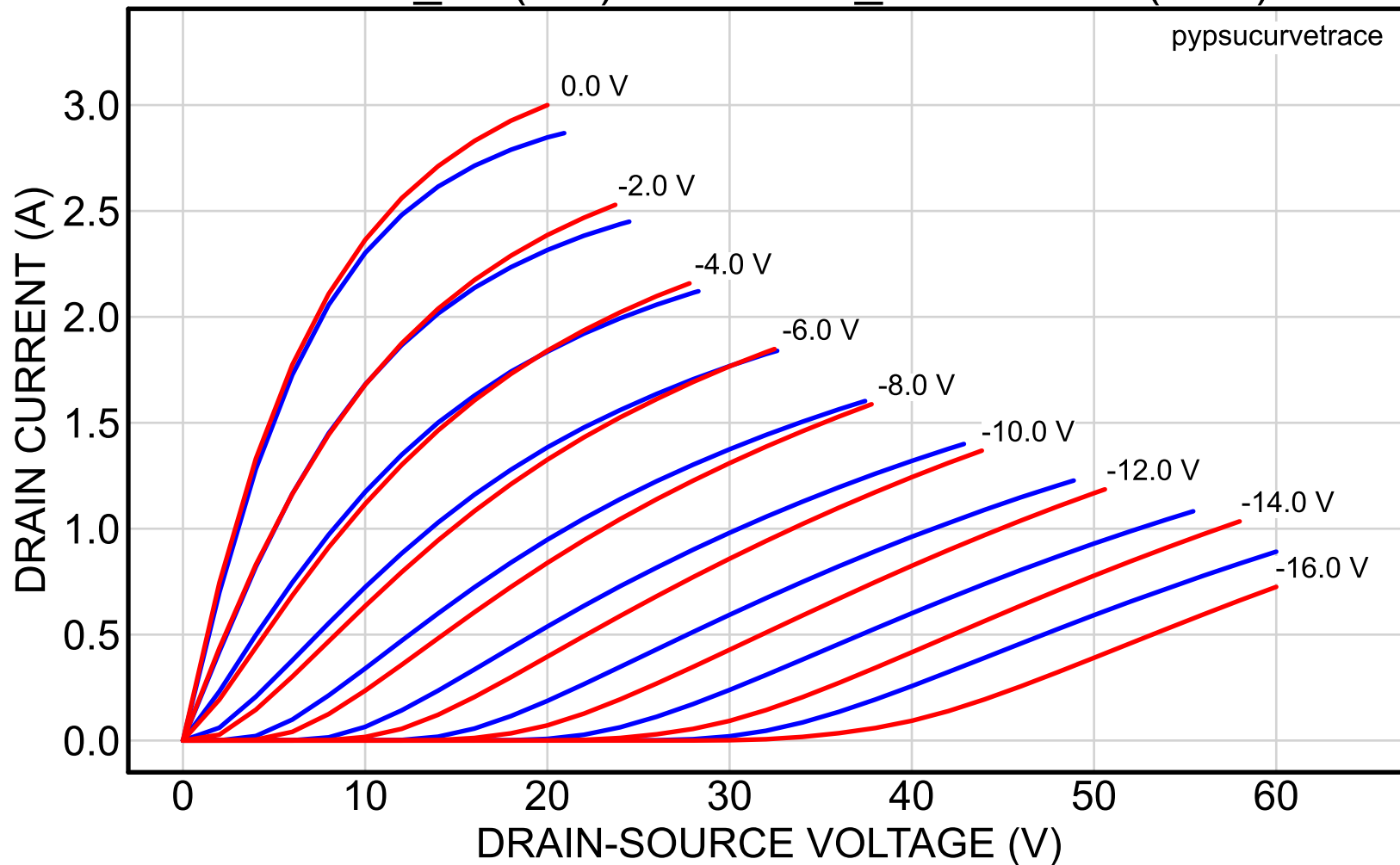
2SK82_20 (red) vs. 2SK82_40reserved (blue)
