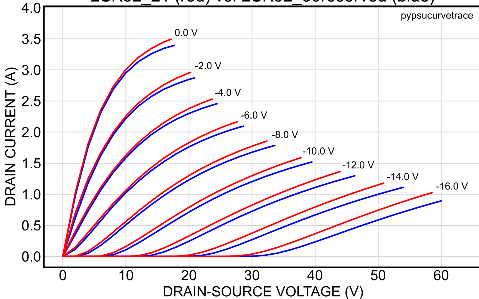
2SK82_21 (red) vs. 2SK82_39reserved (blue)
