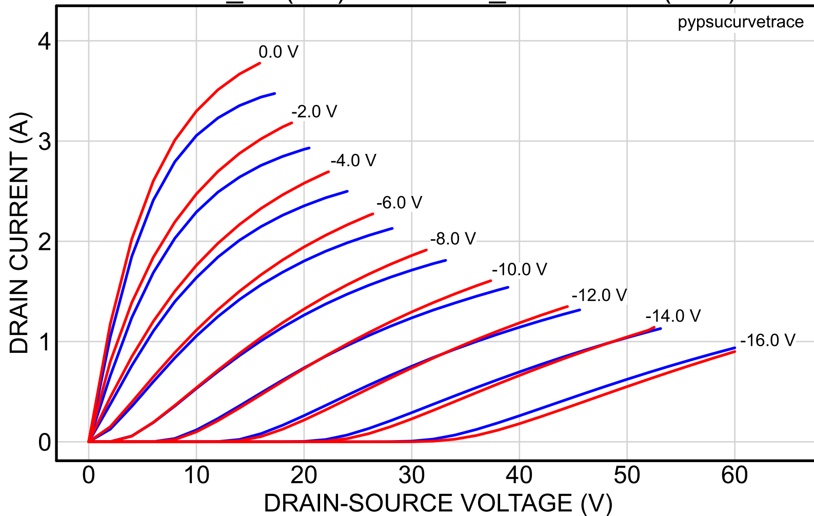
2SK82_22 (red) vs. 2SK82_52reserved (blue)
