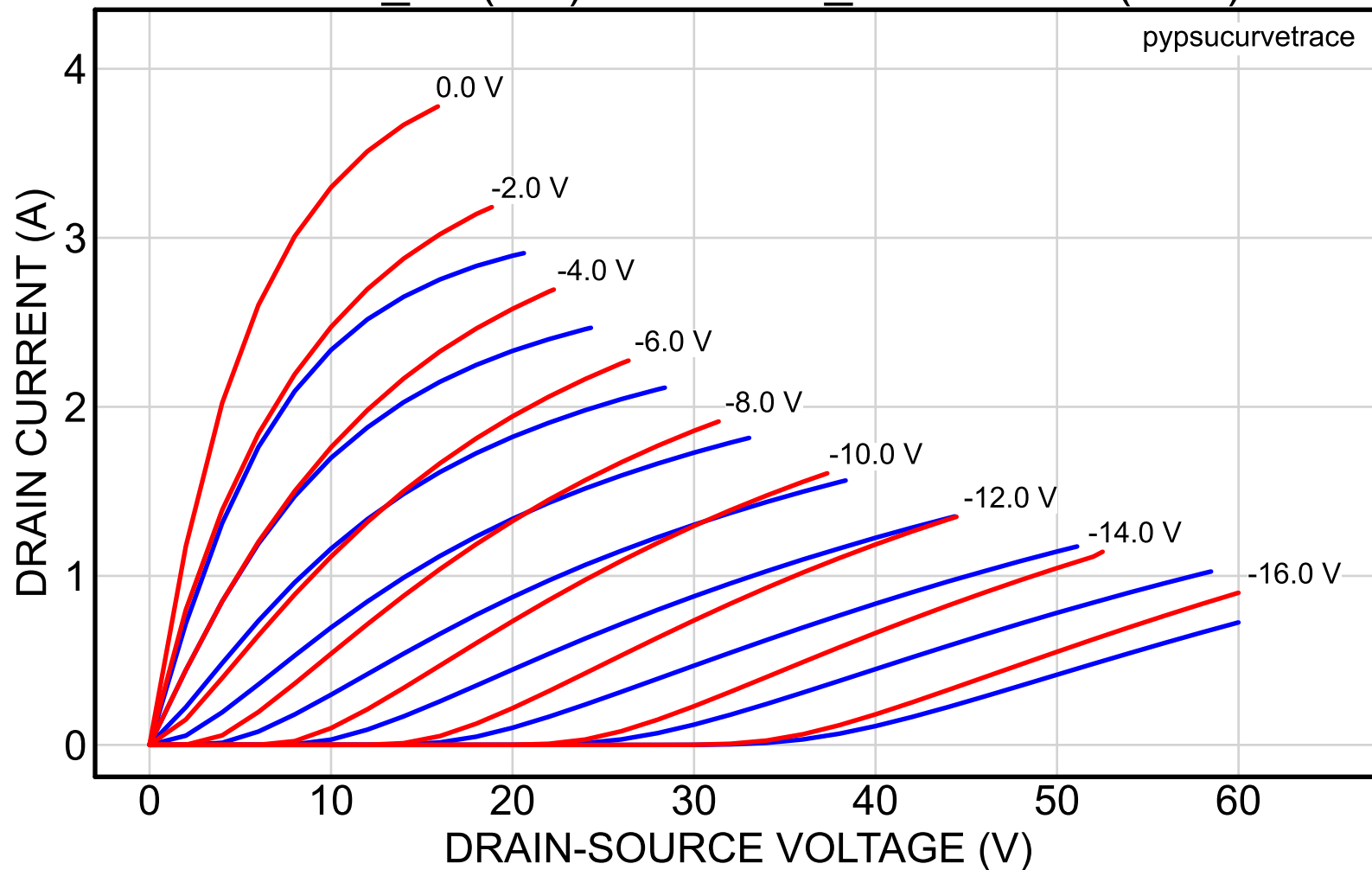
2SK82_22 (red) vs. 2SK82_56reserved (blue)
