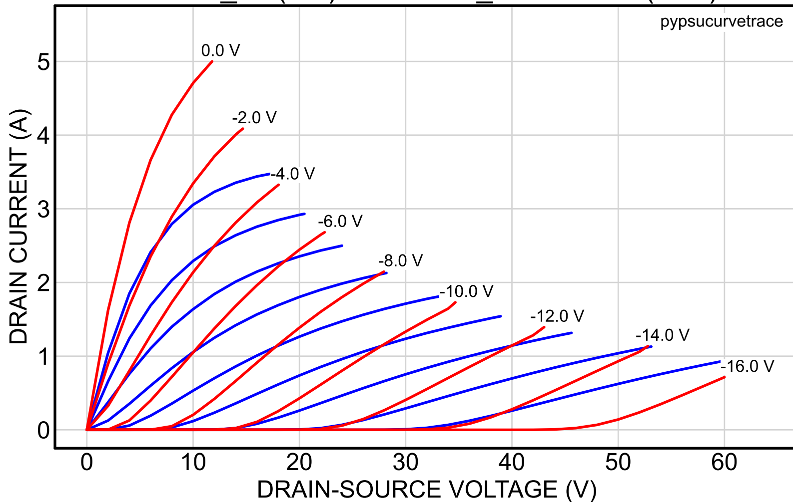
2SK82_23 (red) vs. 2SK82_52reserved (blue)
