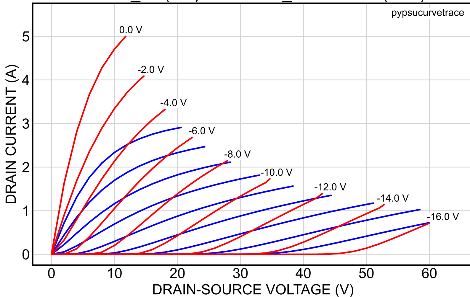
2SK82_23 (red) vs. 2SK82_56reserved (blue)
