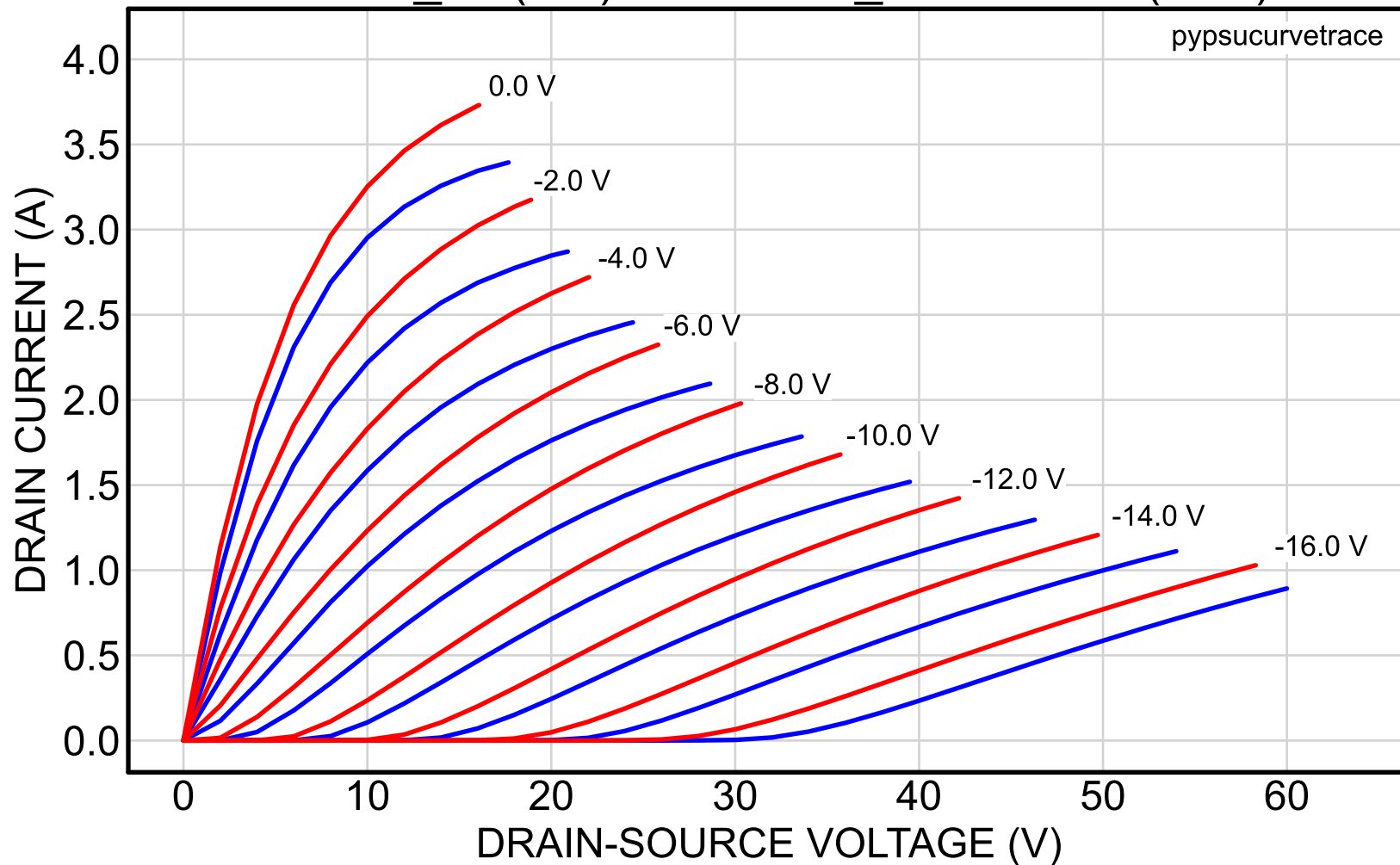
2SK82_24 (red) vs. 2SK82_39reserved (blue)
