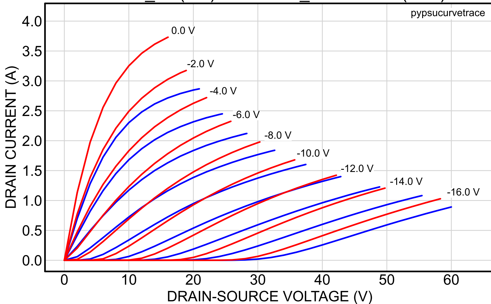
2SK82_24 (red) vs. 2SK82_40reserved (blue)
