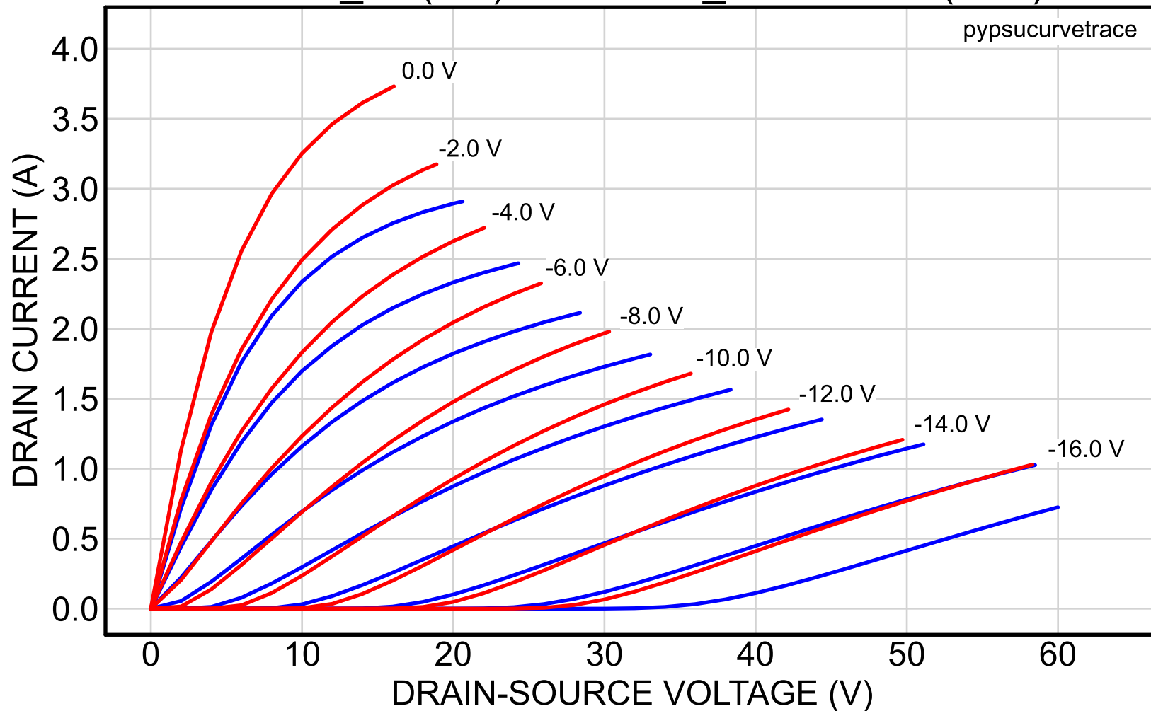
2SK82_24 (red) vs. 2SK82_56reserved (blue)
