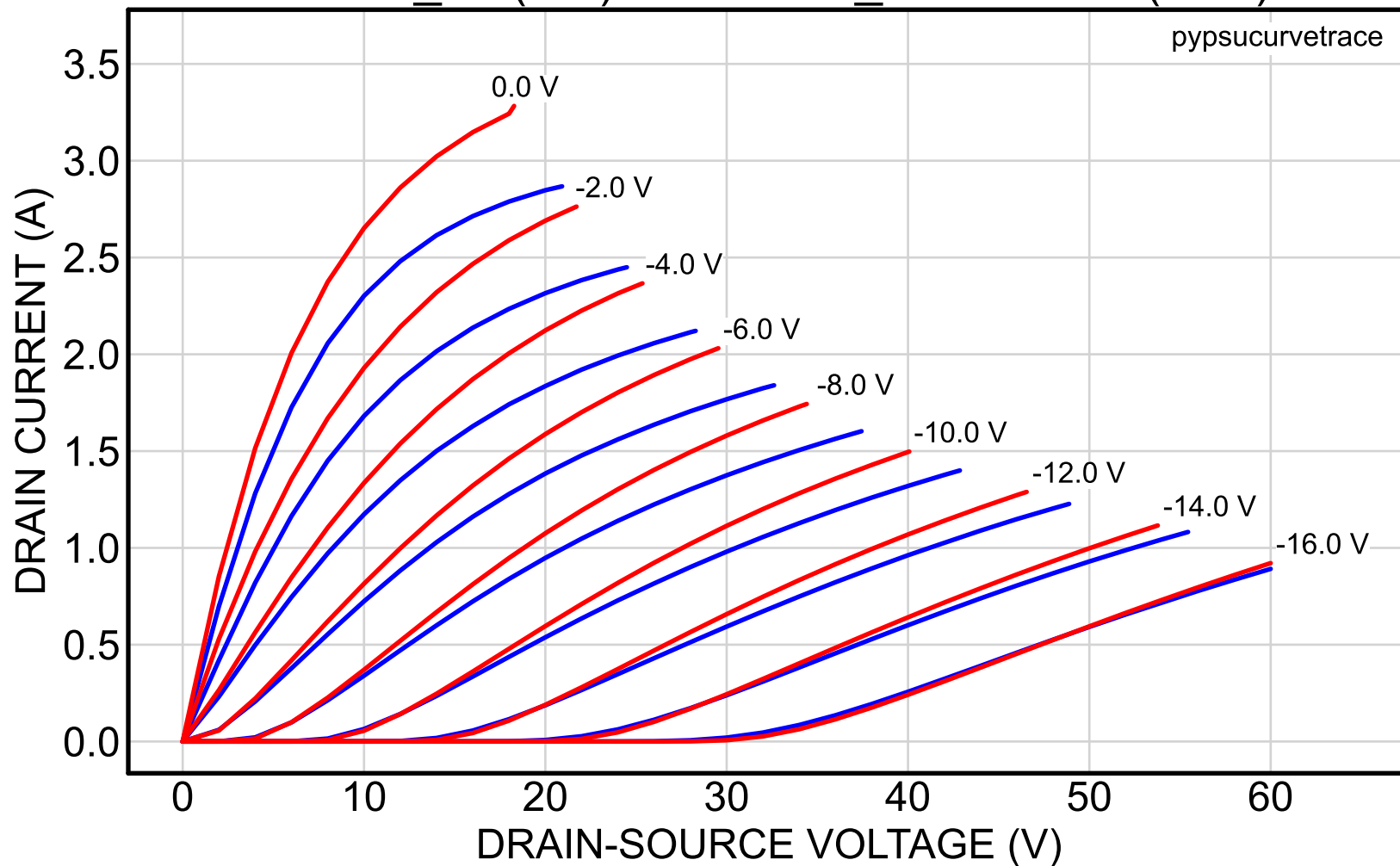
2SK82_25 (red) vs. 2SK82_40reserved (blue)
