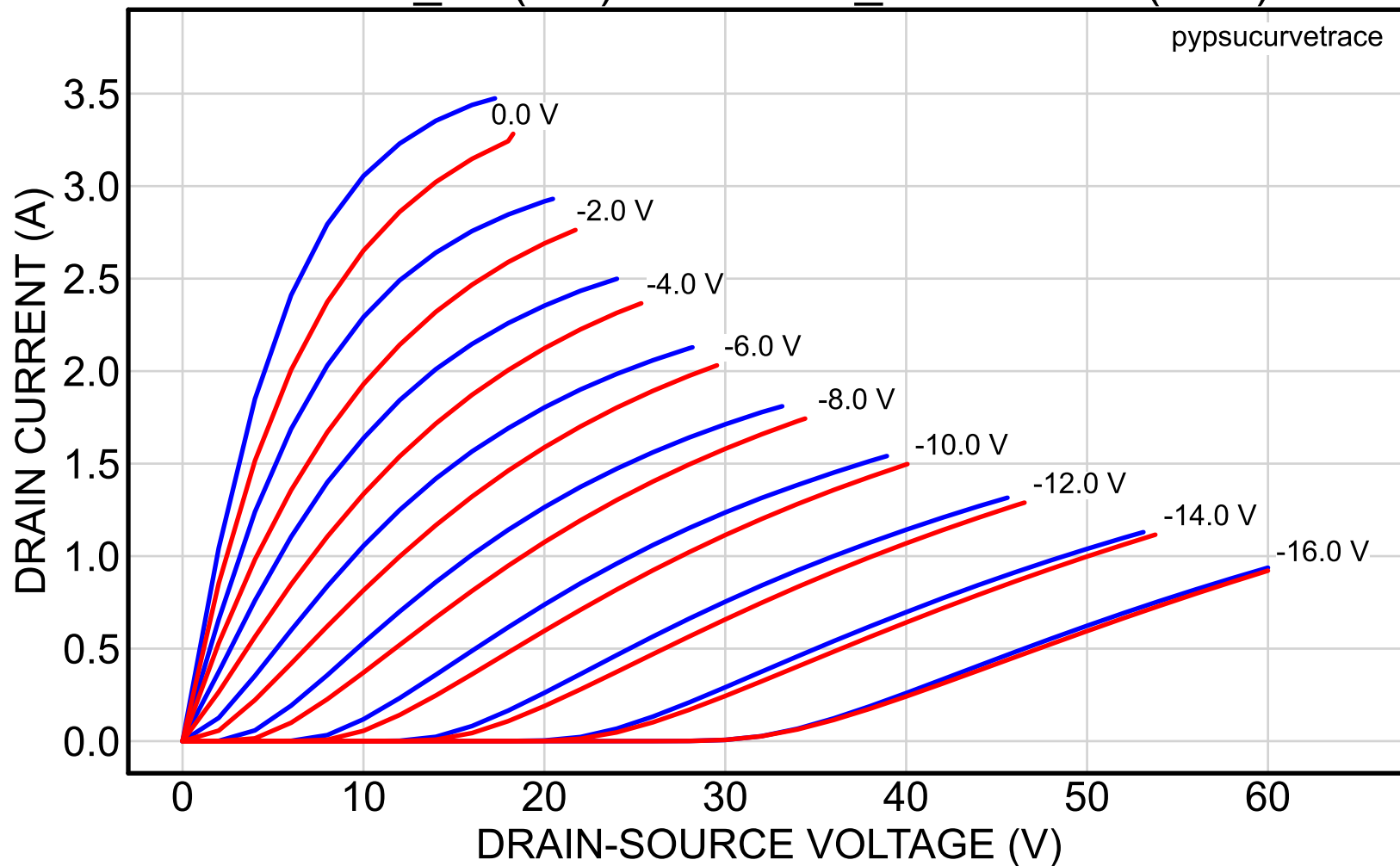
2SK82_25 (red) vs. 2SK82_52reserved (blue)
