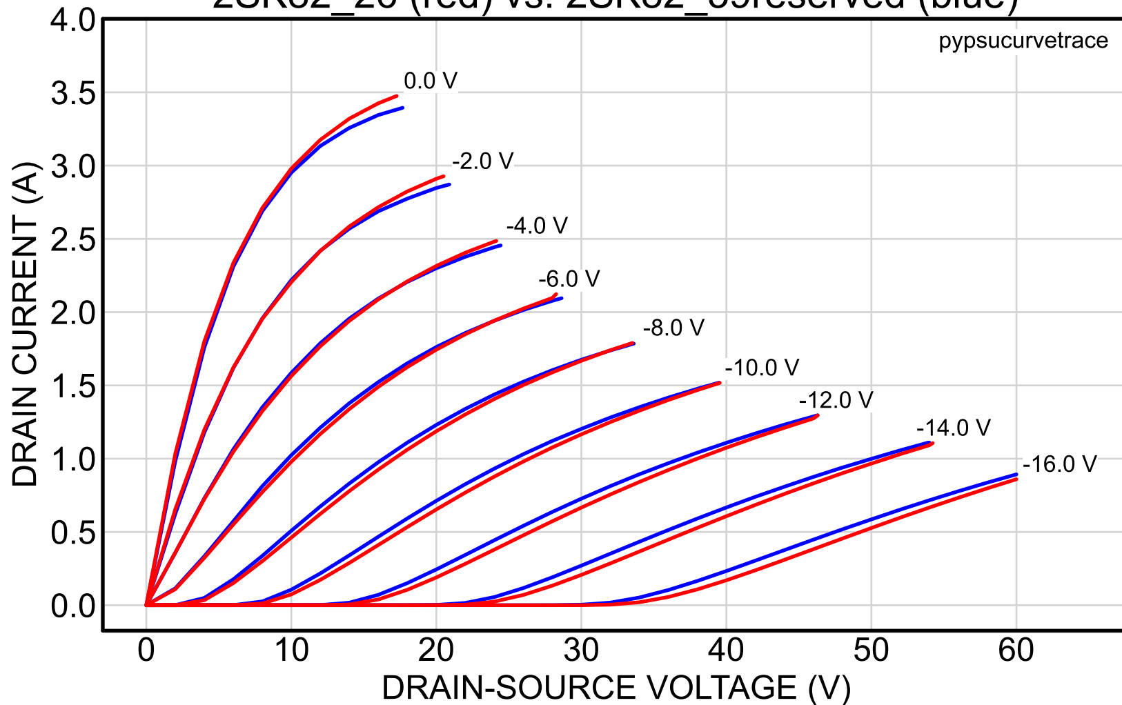
2SK82_26 (red) vs. 2SK82_39reserved (blue)
