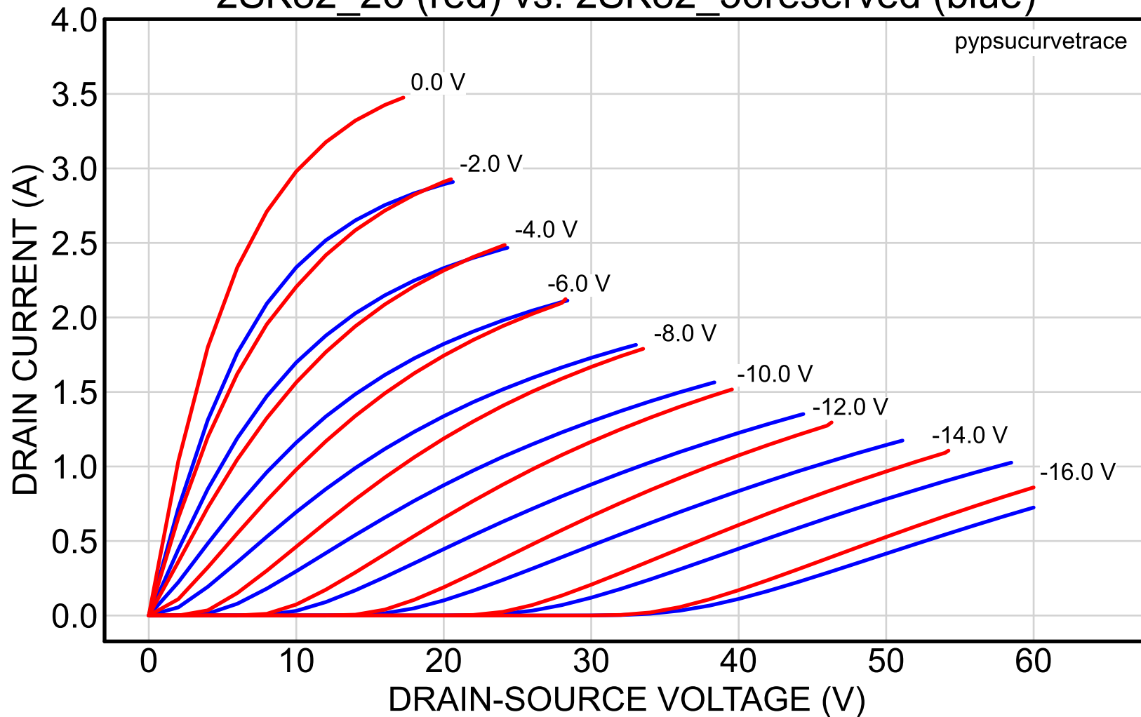
2SK82_26 (red) vs. 2SK82_56reserved (blue)
