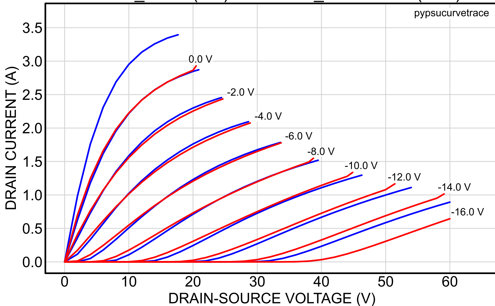
2SK82_27NA (red) vs. 2SK82_39reserved (blue)
