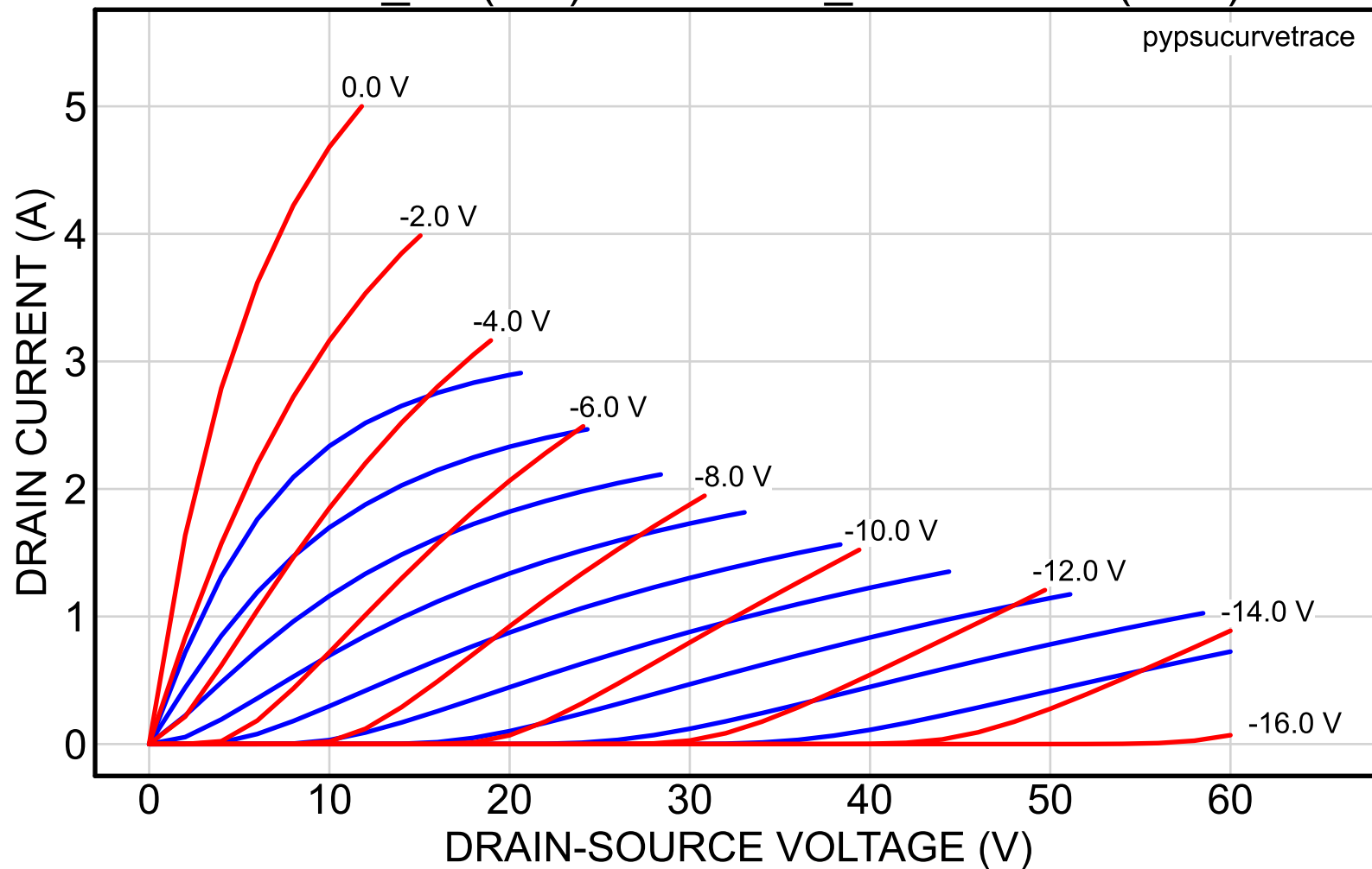
2SK82_28 (red) vs. 2SK82_56reserved (blue)
