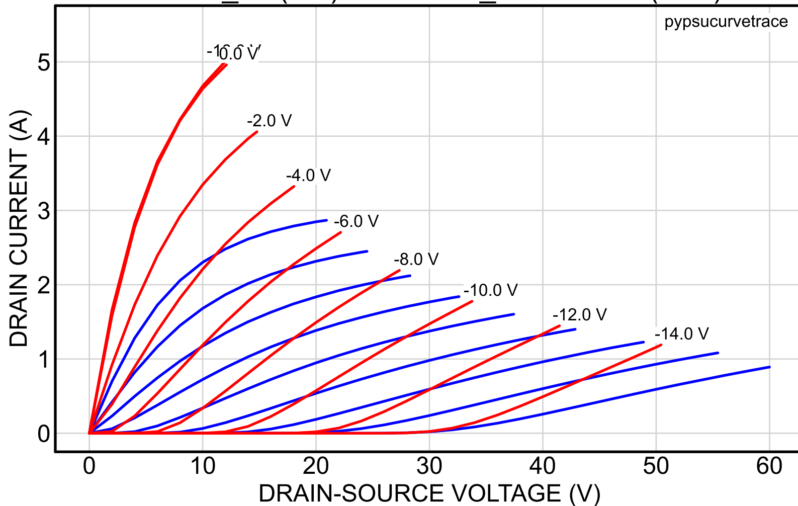
2SK82_29 (red) vs. 2SK82_40reserved (blue)
