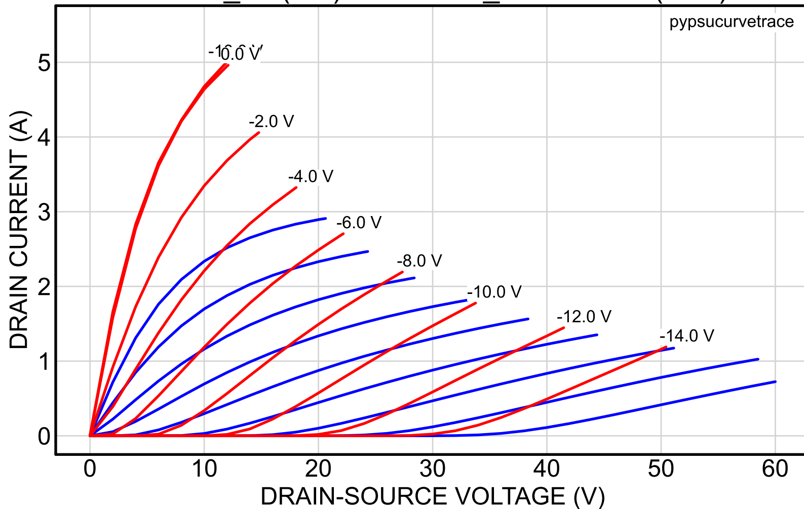
2SK82_29 (red) vs. 2SK82_56reserved (blue)
