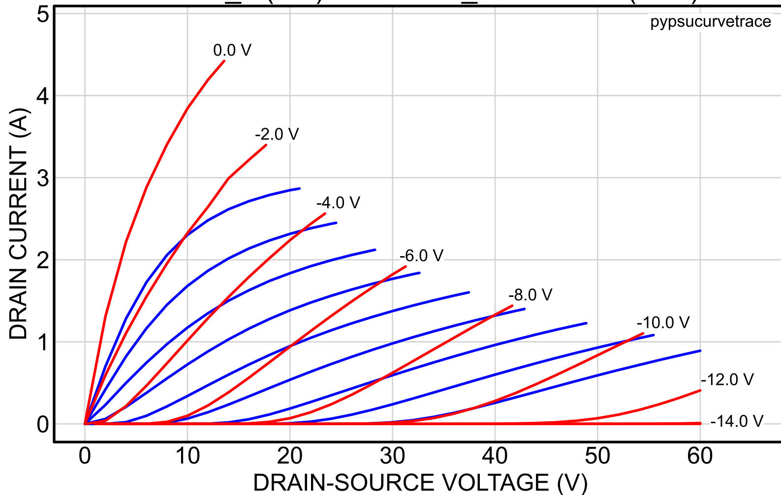
2SK82_2 (red) vs. 2SK82_40reserved (blue)
