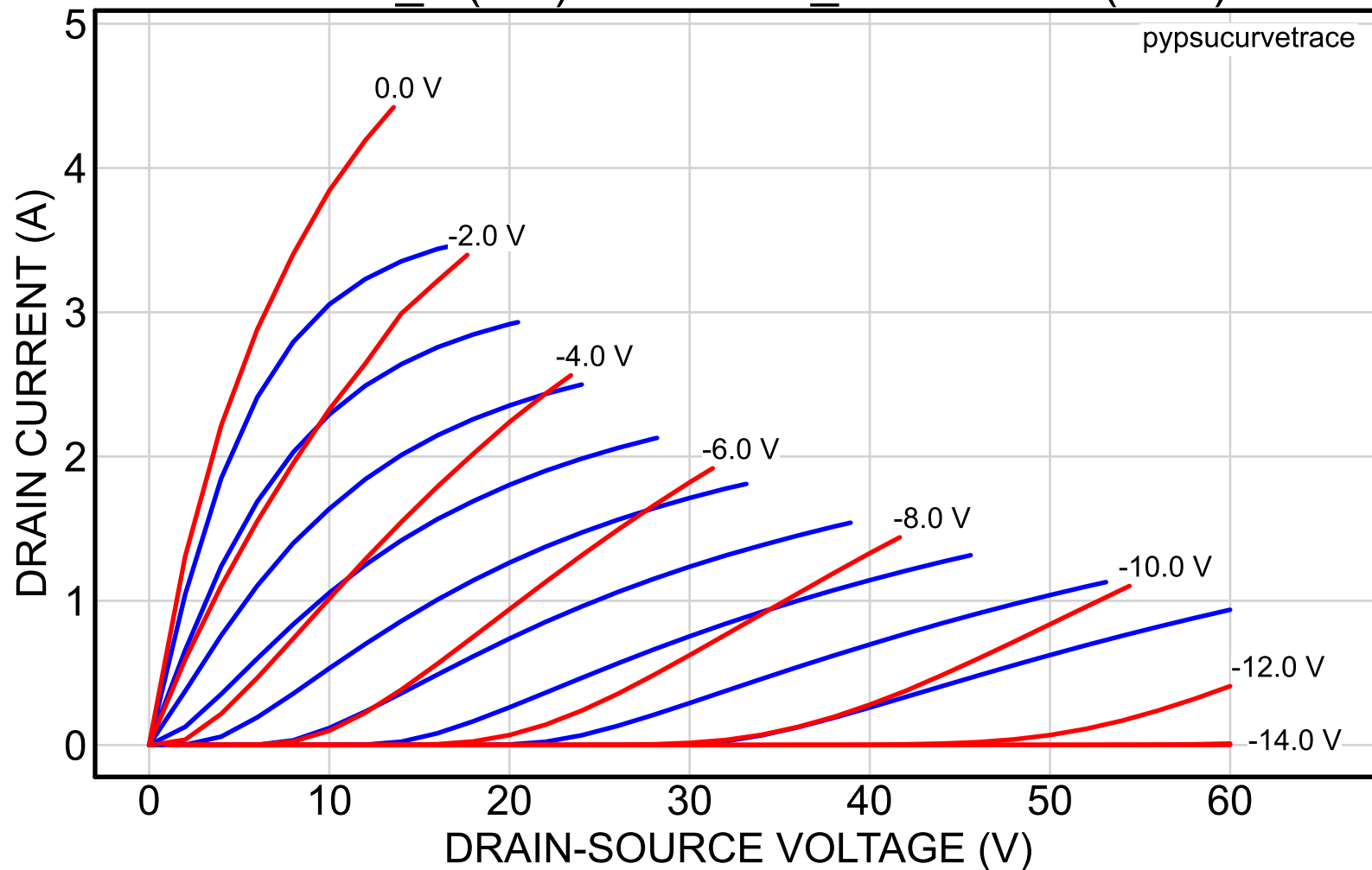
2SK82_2 (red) vs. 2SK82_52reserved (blue)
