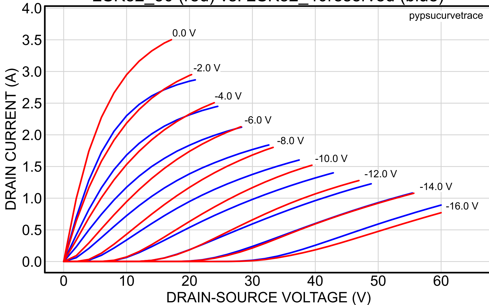
2SK82_30 (red) vs. 2SK82_40reserved (blue)
