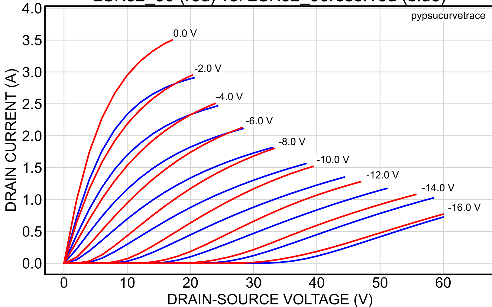
2SK82_30 (red) vs. 2SK82_56reserved (blue)
