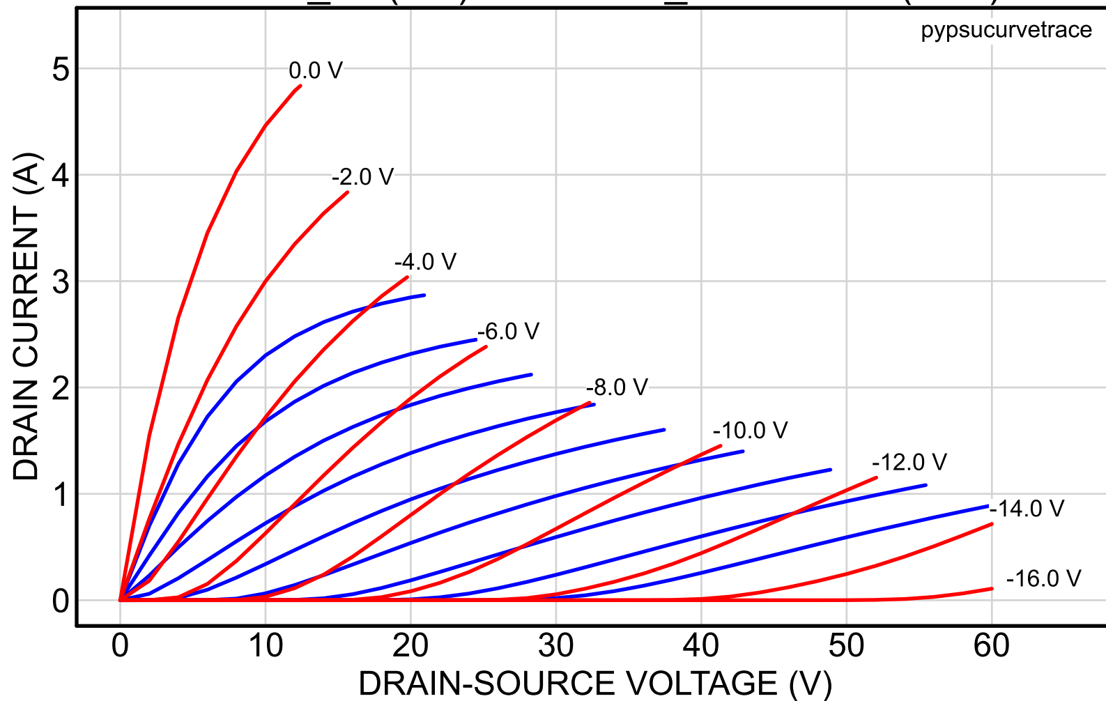
2SK82_31 (red) vs. 2SK82_40reserved (blue)
