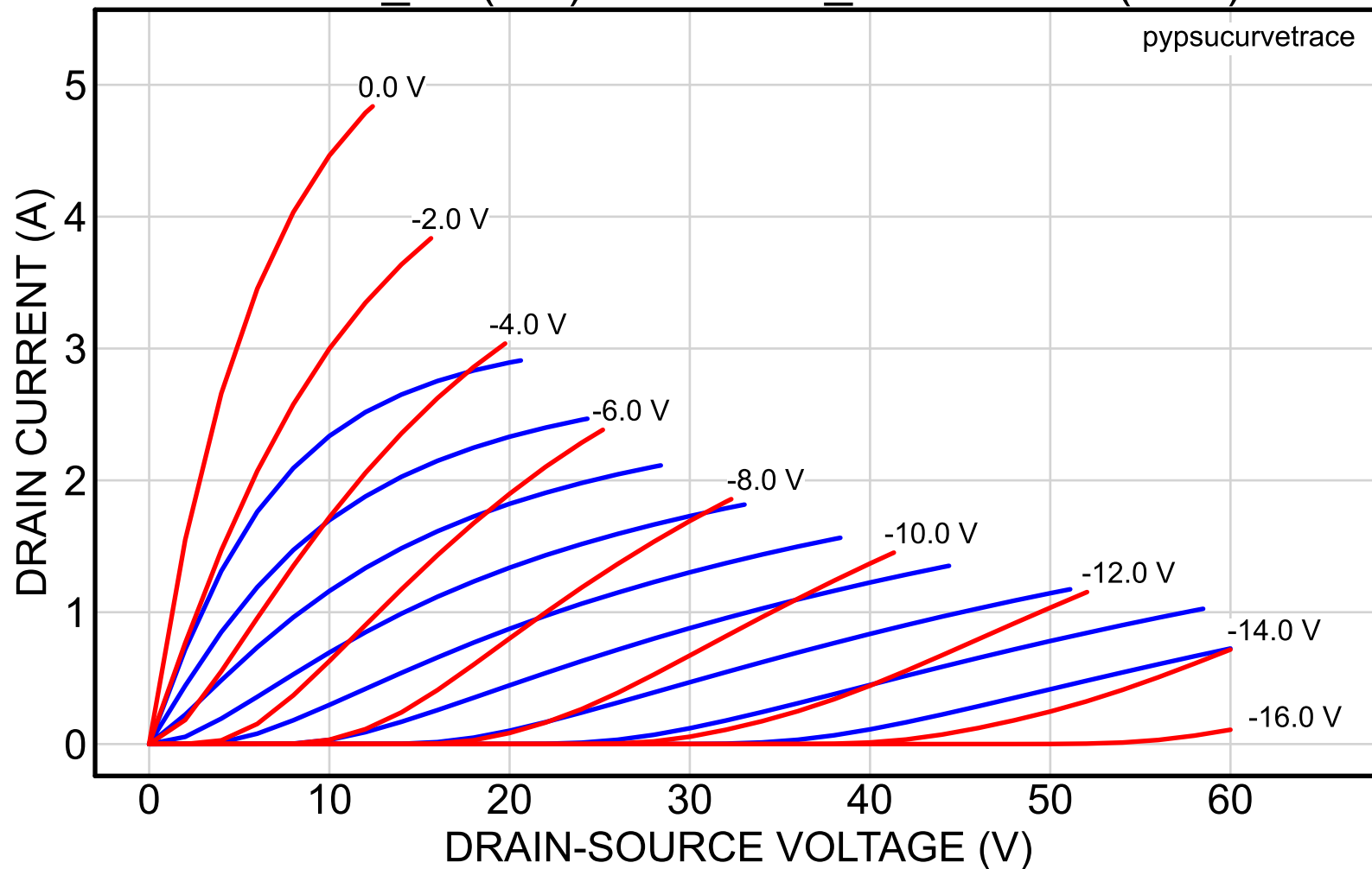
2SK82_31 (red) vs. 2SK82_56reserved (blue)
