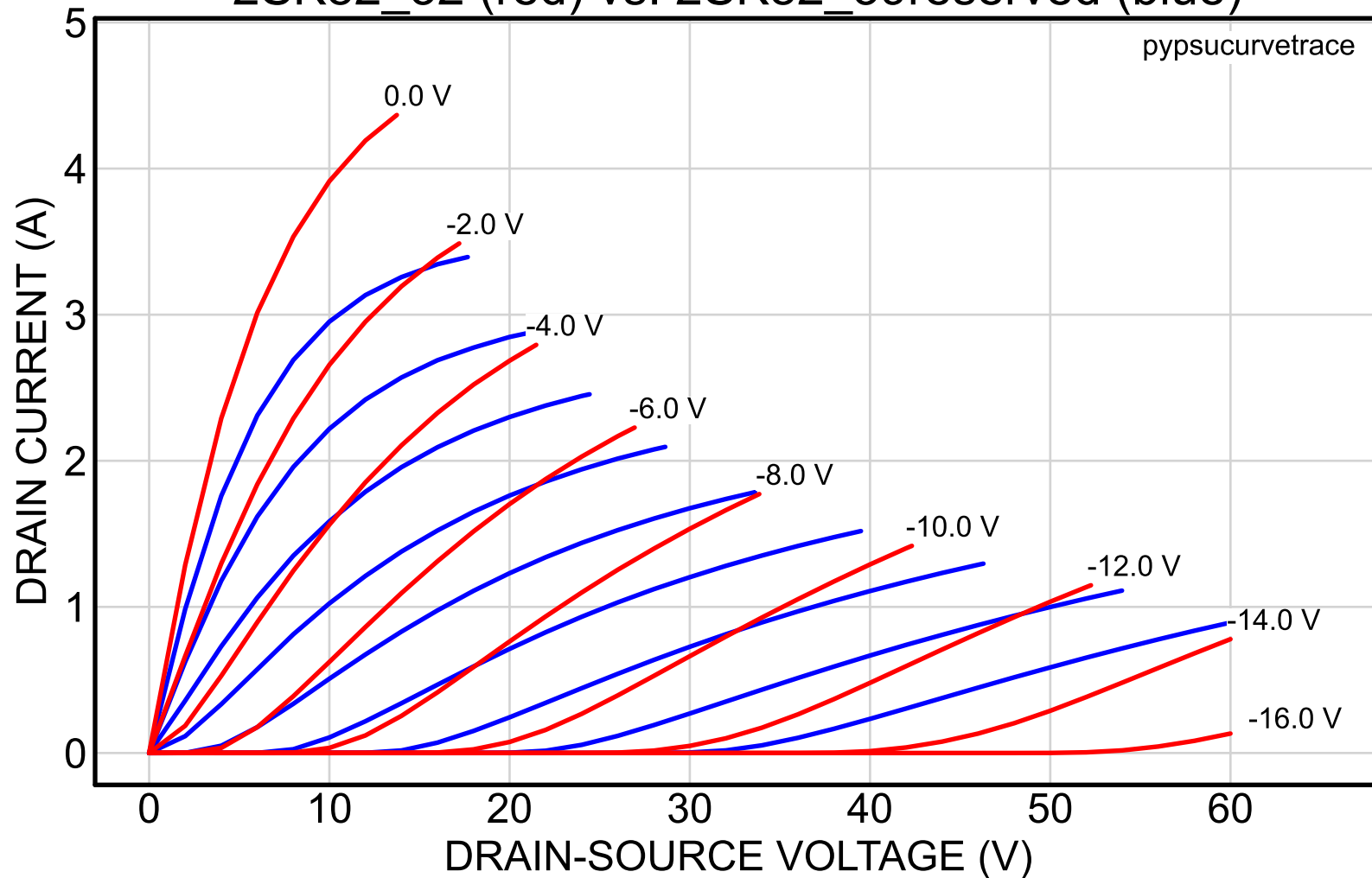
2SK82_32 (red) vs. 2SK82_39reserved (blue)
