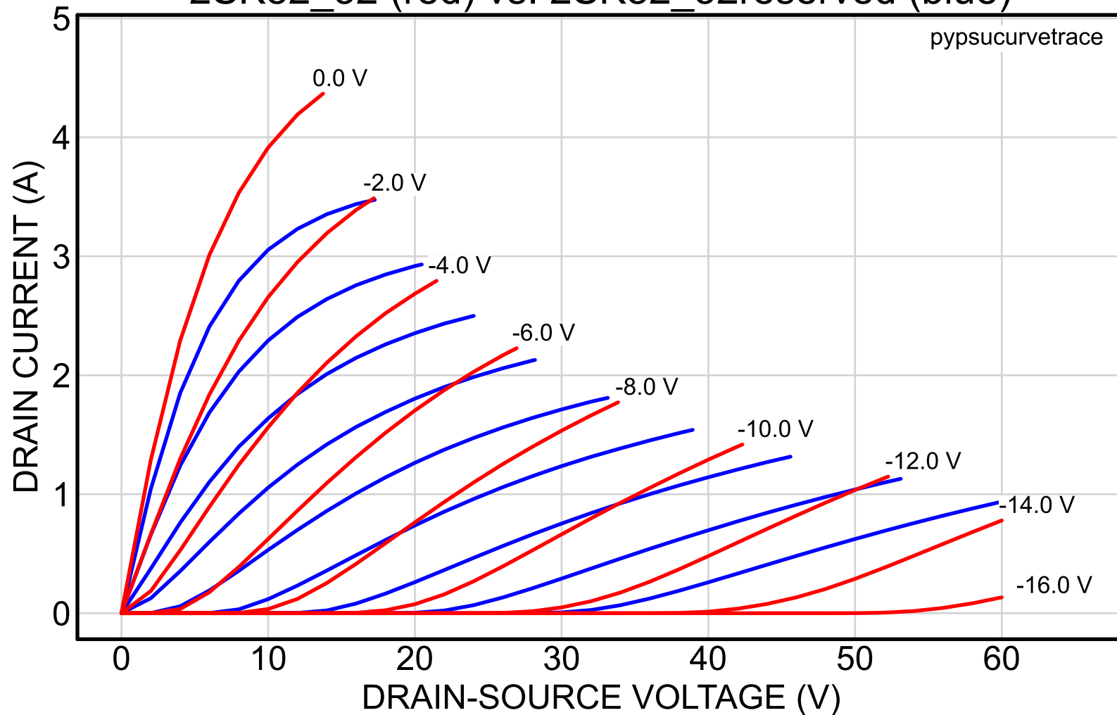
2SK82_32 (red) vs. 2SK82_52reserved (blue)
