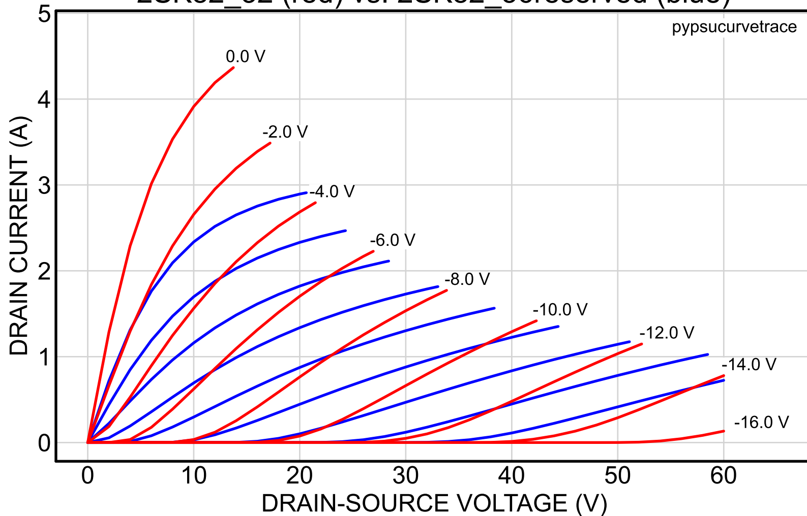
2SK82_32 (red) vs. 2SK82_56reserved (blue)
