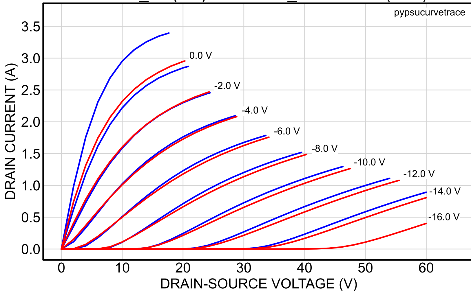
2SK82_34 (red) vs. 2SK82_39reserved (blue)
