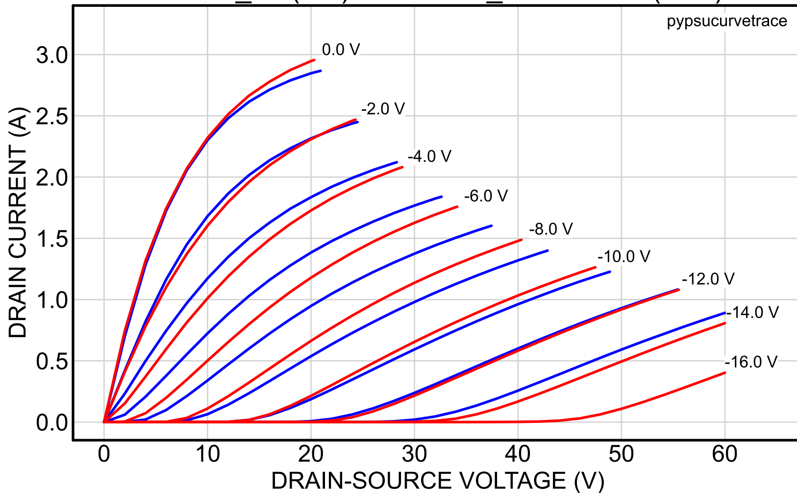
2SK82_34 (red) vs. 2SK82_40reserved (blue)
