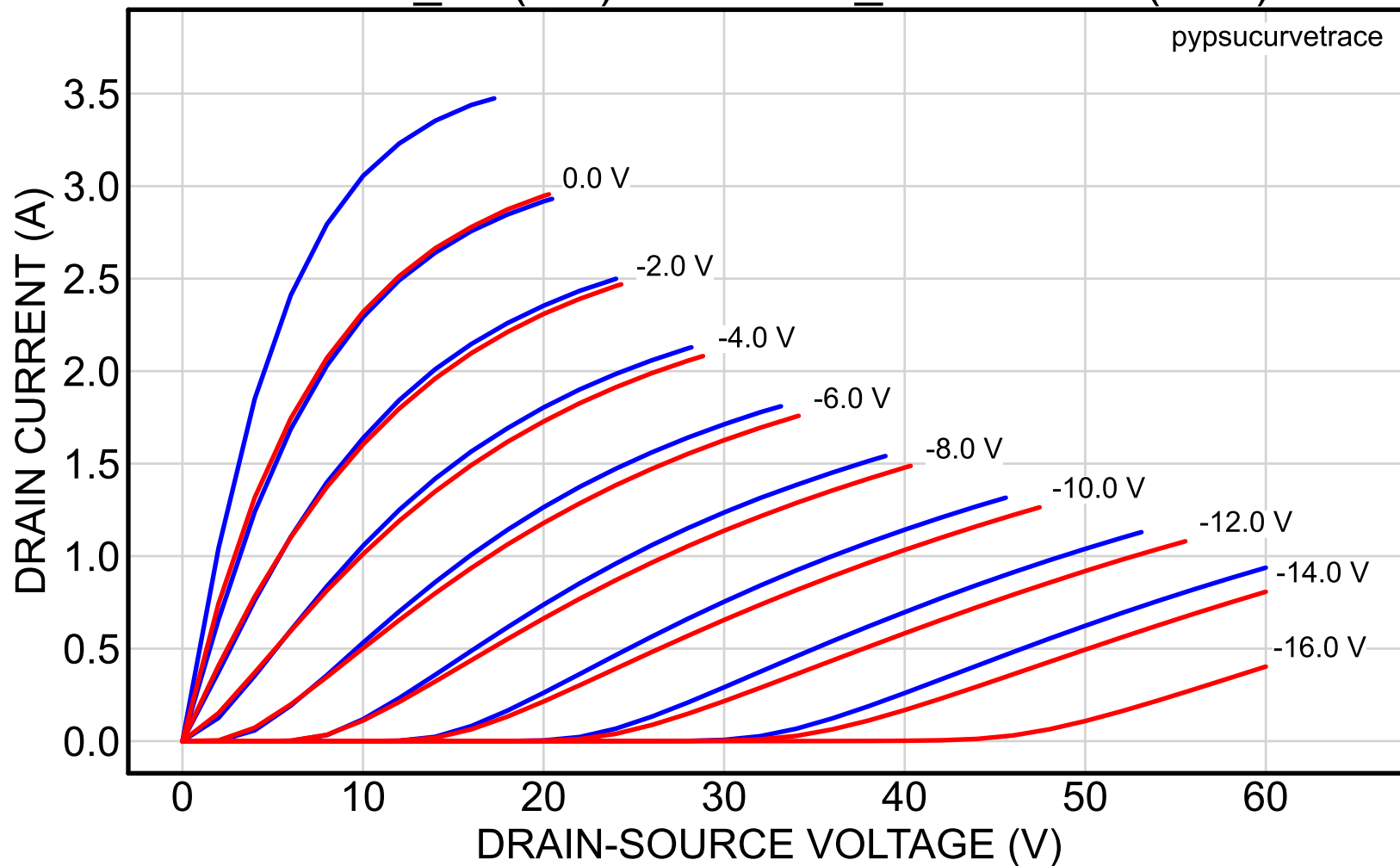
2SK82_34 (red) vs. 2SK82_52reserved (blue)
