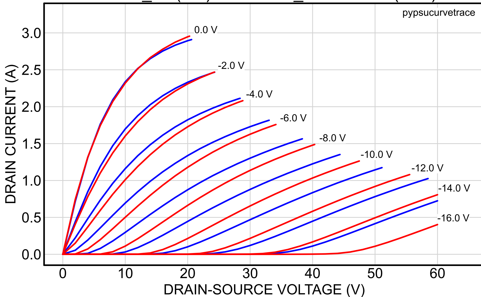
2SK82_34 (red) vs. 2SK82_56reserved (blue)
